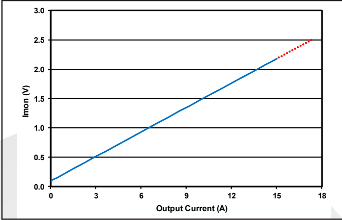
Figure 13: I mon pin Voltage vs. Output Load Current.
